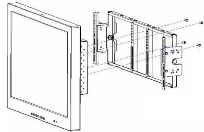
SINGLE MOUNT
