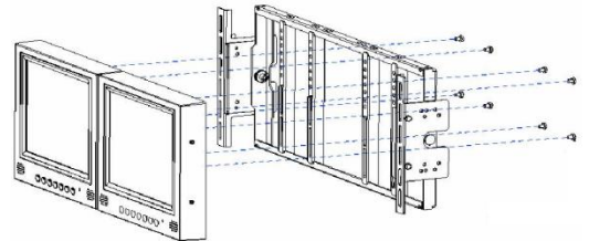
DUAL MOUNT
